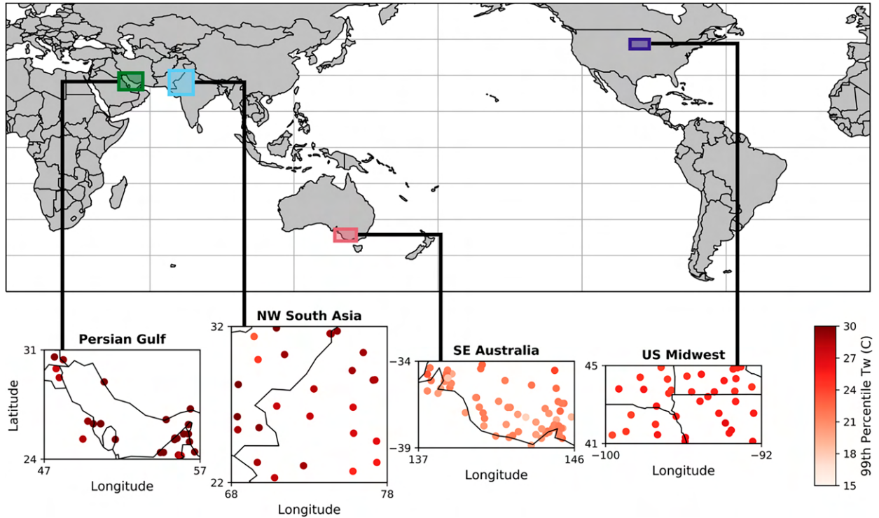
FIG. 1. HadISD station locations included in regional analyses, colored by 99th-percentile daily maximum T_w (full year). Four boxed regions of interest are referred to as Persian Gulf, NW South Asia, SE Australia, and U.S. Midwest.
